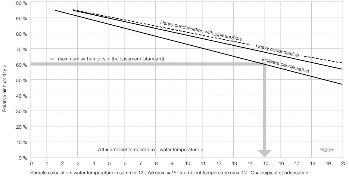
Diagram for the determination of the dew point for POLYMUTAN SDR 6
